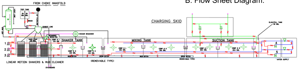
B. Flow Sheet Diagram.
